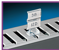
Designed for use with several accessories: wire retainers, label holders etc.
